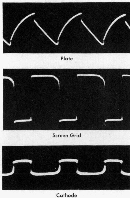
Figure 3B. Waveforms Observed at Tube Electrodes.
